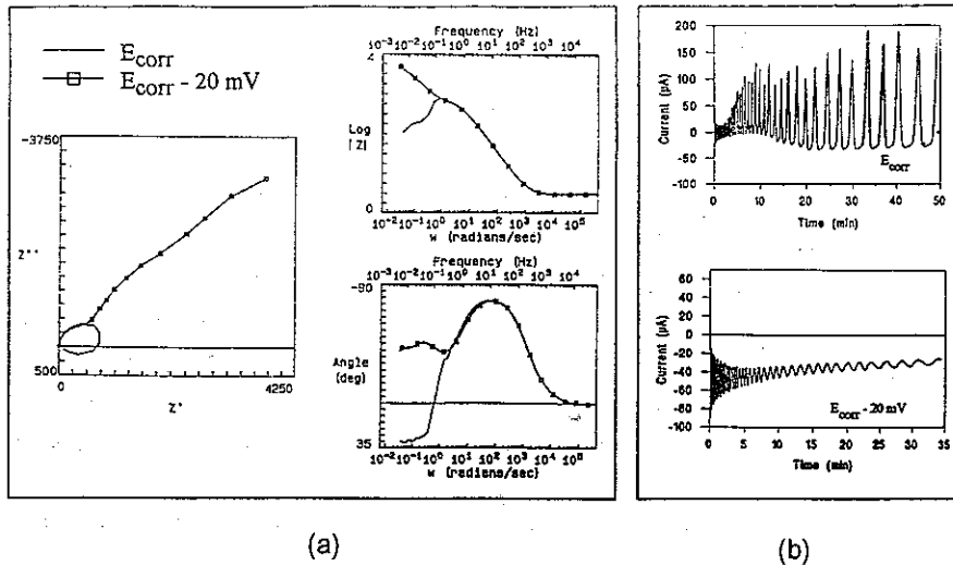
FIG.1 - Impedance spectra (a) and current vs time plot (b) at E_{CORR} and E_{CORR} - 20 \text{ mV} for 1 h of immersion.
